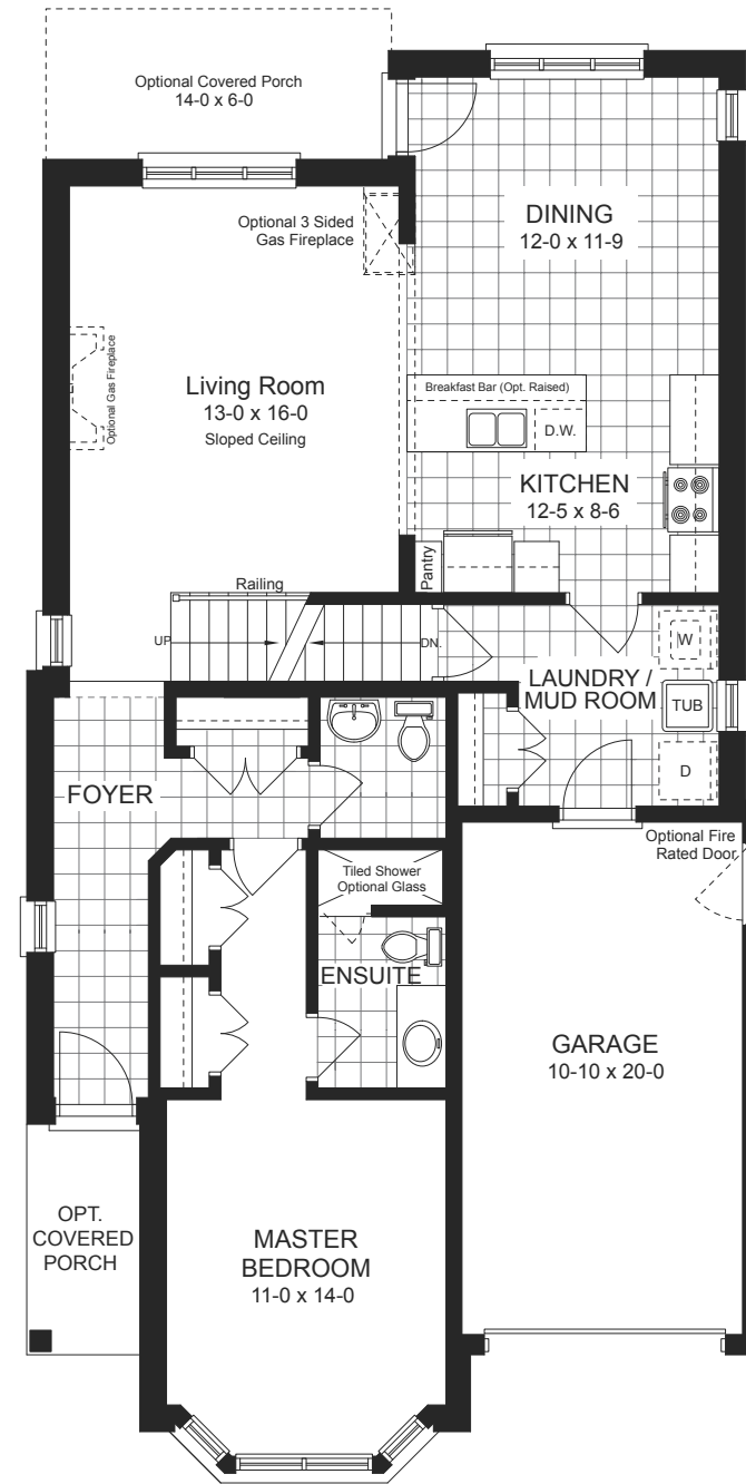
MAIN FLOOR ELEVATION A ALTERNATE LAYOUT 1. OPT. COVERED PORCH
