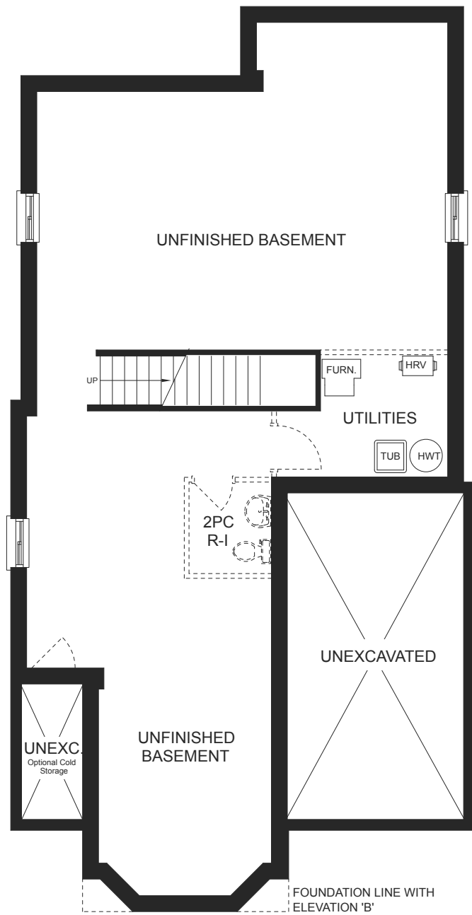
BASEMENT
