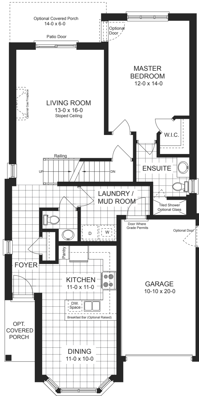
MAIN FLOOR ELEVATION A STANDARD LAYOUT 1. OPT. COVERED PORCH
