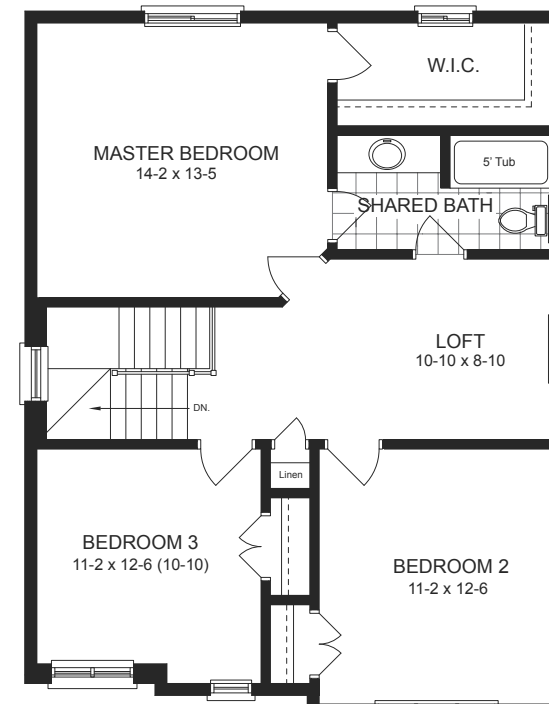
4. ALT. SECOND FLOOR ELEVATION A LOFT LAYOUT
