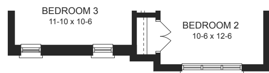
SECOND FLOOR ELEVATION B
