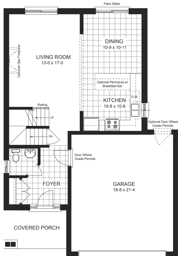
MAIN FLOOR ELEVATION A
