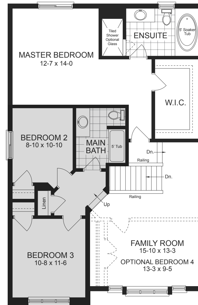
SECOND FLOOR ELEVATION A 3. OPT. 4 BEDROOM LAYOUT
