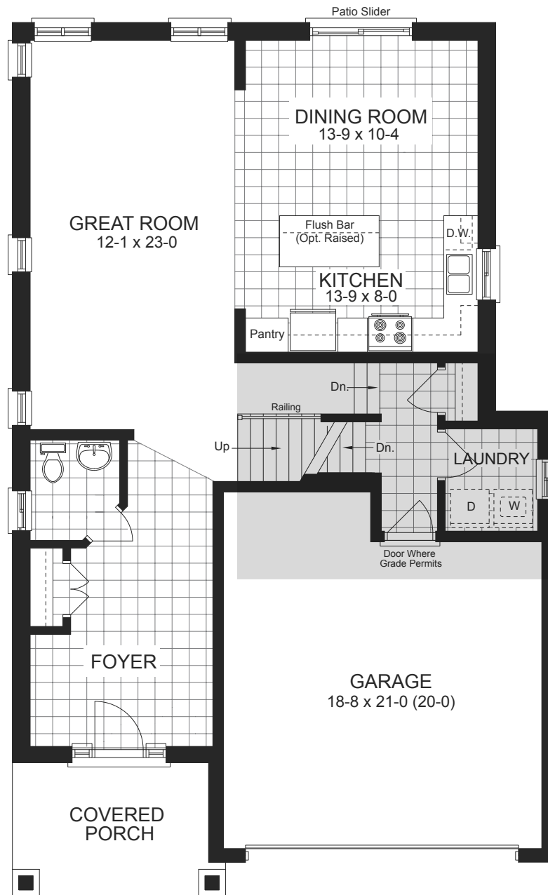
MAIN FLOOR ELEVATION A & B
