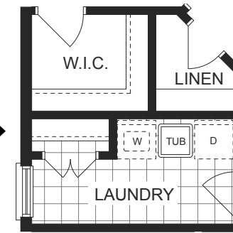
2. OPT. SECOND FLOOR LAUNDRY LAYOUT
