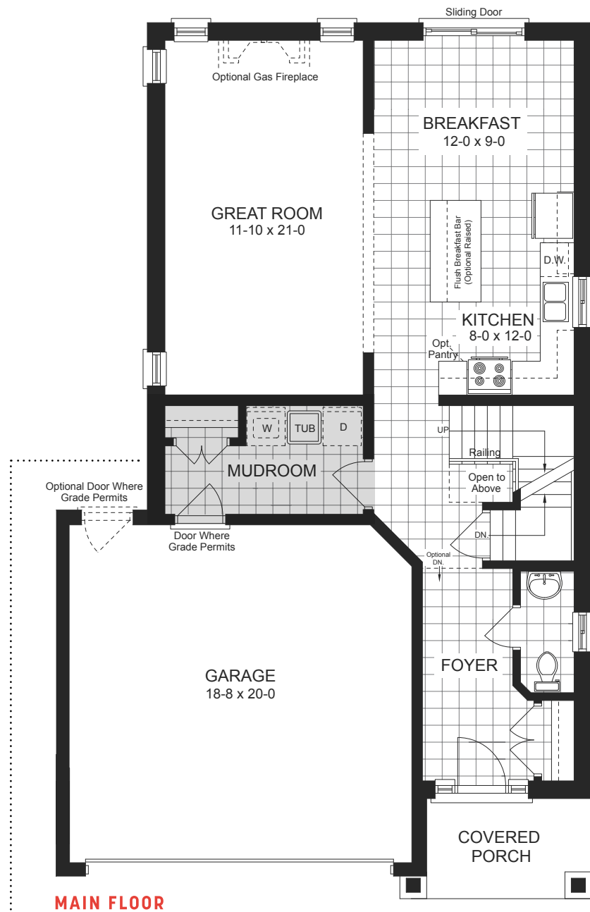
MAIN FLOOR ELEVATION A & B STANDARD LAYOUT
